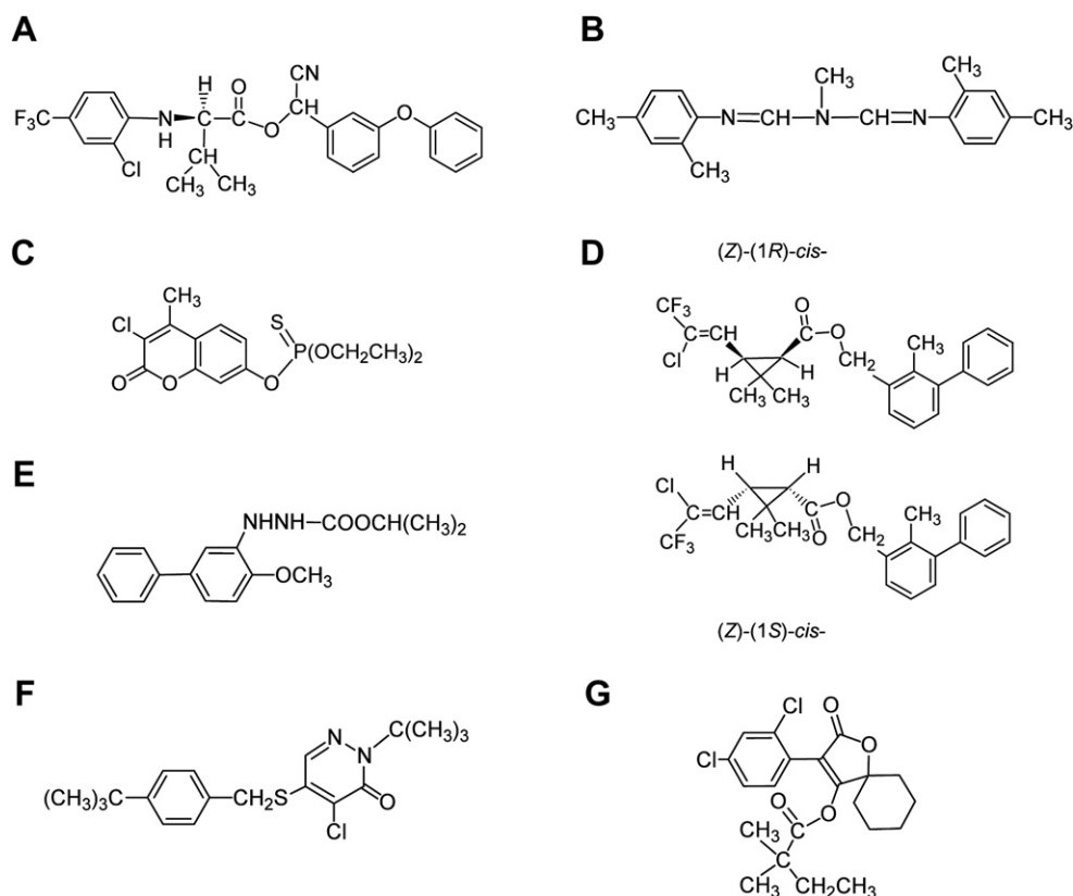
Fig. 1. Chemical structures of economically important acaricides. A) tau-fluvalinate; B) amitraz; C) coumaphos; D) bifenthrin; E) bifenazate; F) pyridaben; G) spiroadiclofen.
